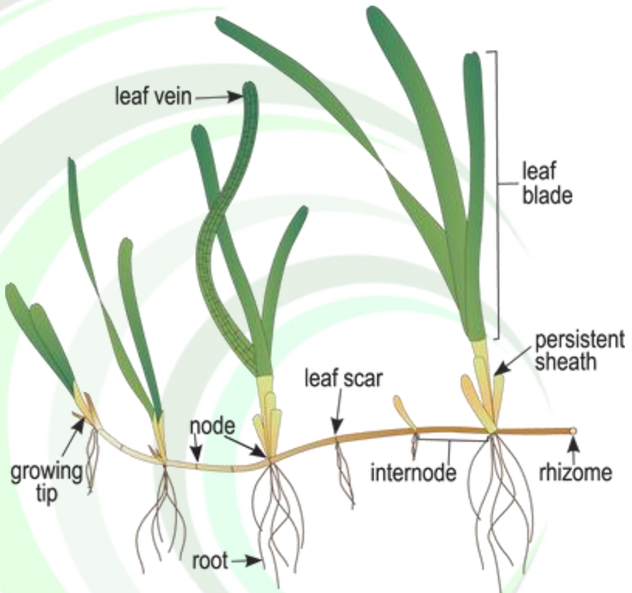
Conceptual diagram illustrating the morphology of Zostera capensis (marine eelgrass). Diagram courtesy of James Cook University, Australia.
